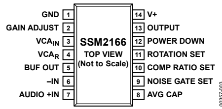
Figure 3. Pin Configuration
