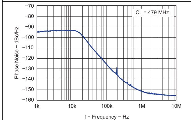
Figure 51. Closed Loop VCO Phase Noise
