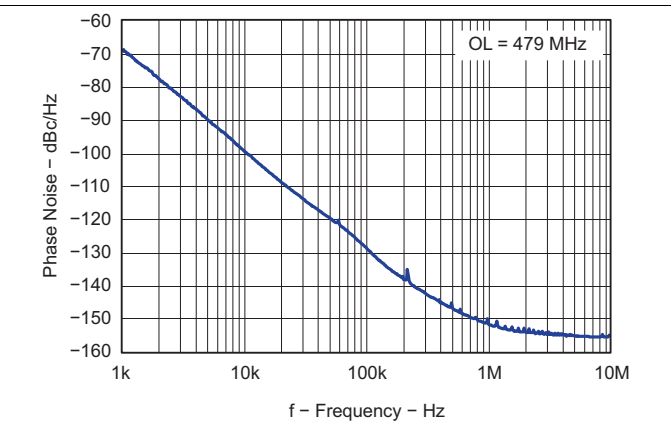
Figure 52. Open Loop VCO Phase Noise
