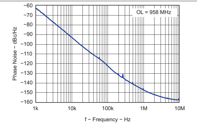
Figure 50. Open Loop VCO Phase Noise
