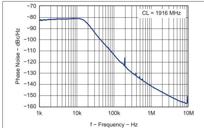
Figure 47. Closed Loop VCO Phase Noise
