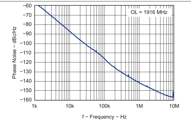
Figure 48. Open Loop VCO Phase Noise
