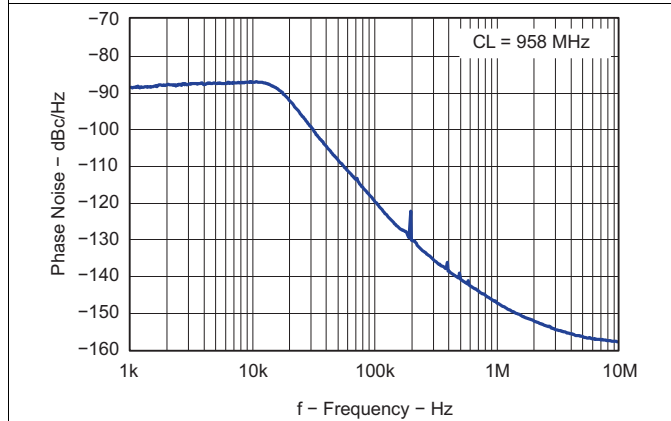
Figure 49. Closed Loop VCO Phase Noise
