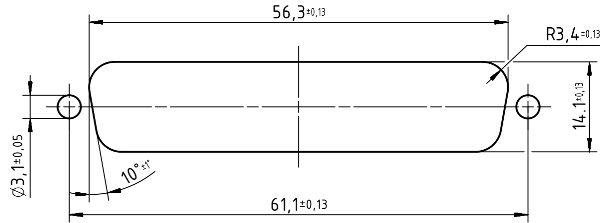
Rear mounting panel cut out
