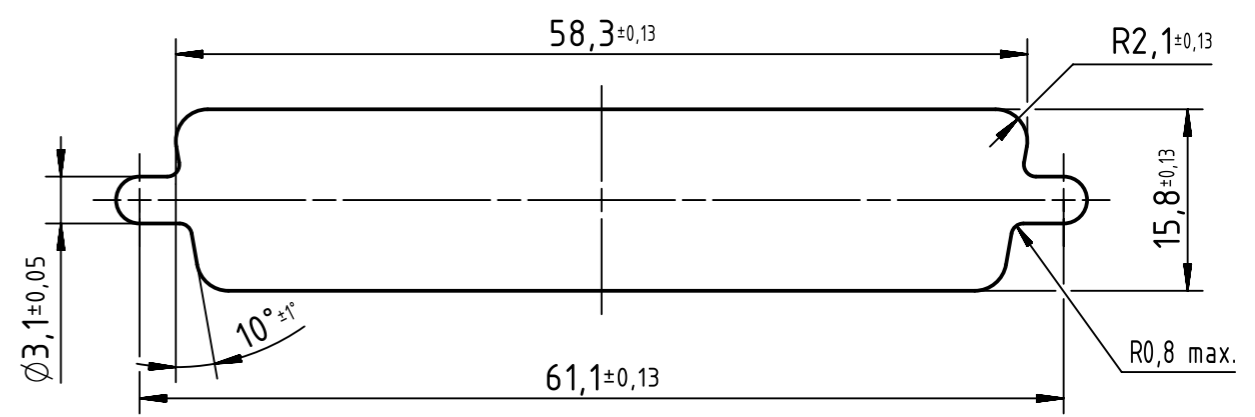
Front mounting panel cut out
