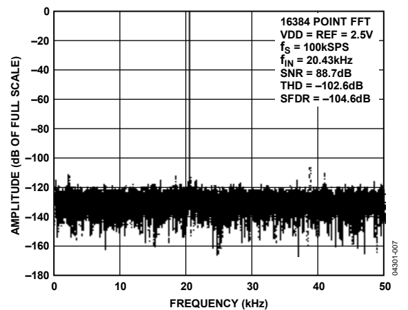
Figure 13. FFT Plot
