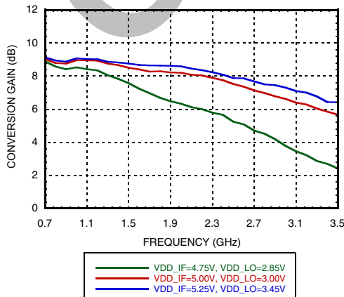
Figure 41. Conversion Gain vs. Vdd @ VGATE=4.8V [1]
