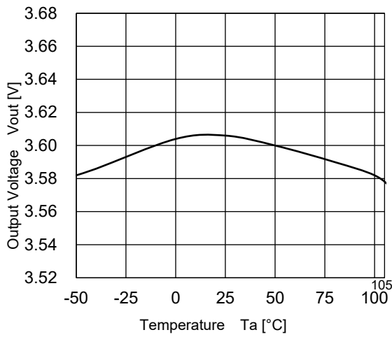
R1180x361x ( V_{IN}=4.6V )
