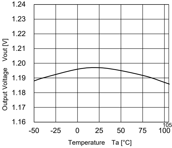
R1180x361x ( V_{IN}=4.6V )
