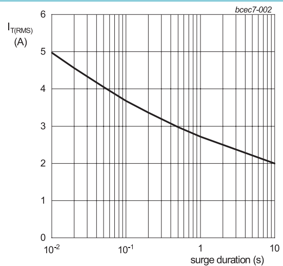
Fig. 2. RMS on-state current as a function of surge duration; maximum values f = 50 Hz; T_{lead} = 57\text{ °C}
