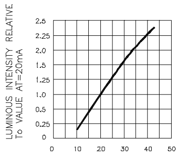
If-FORWARD CURRENT-mA
