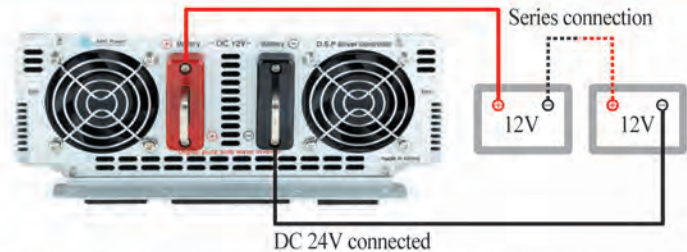
Pure sine wave inverter
