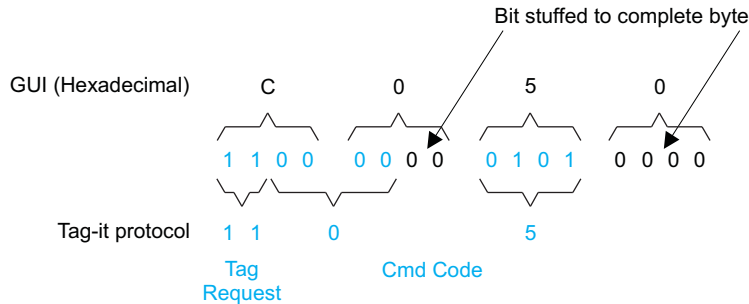
Figure 3-5. Put Block Response Packet Structure
