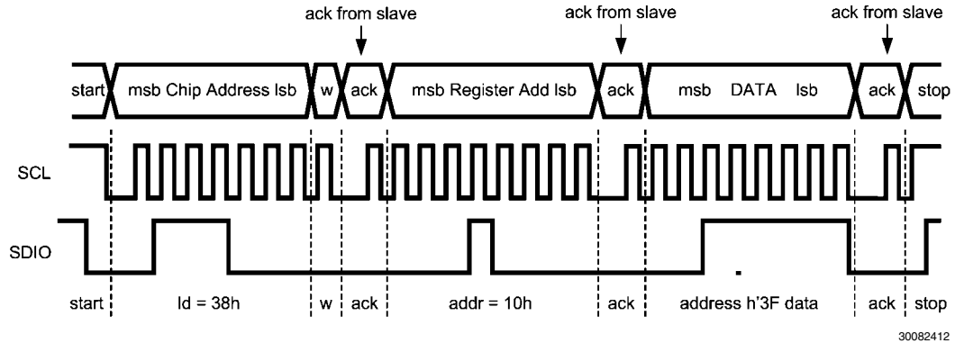
FIGURE 3. Write Cycle w = write (SDIO = "0") r = read (SDIO = "1") ack = acknowledge (SDIO pulled down by either master or slave) id = chip address, 38h for LM3535
