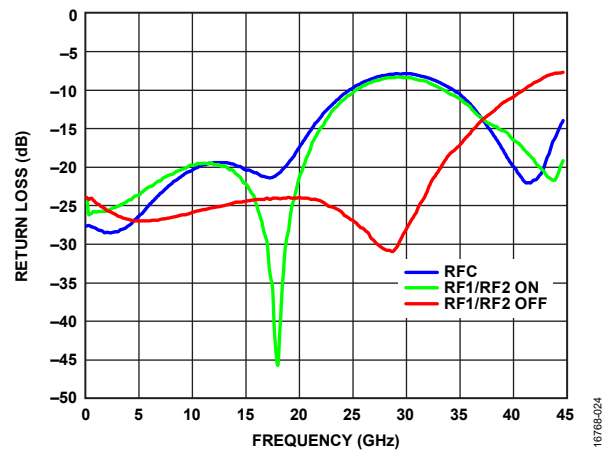
Figure 24. Return Loss vs. Frequency, with Impedance Matching
