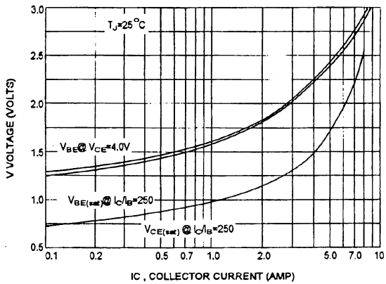
"ON" VOLTAGES
