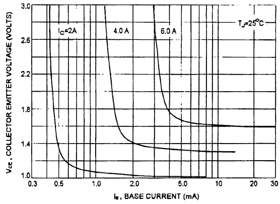
"ON" VOLTAGES
