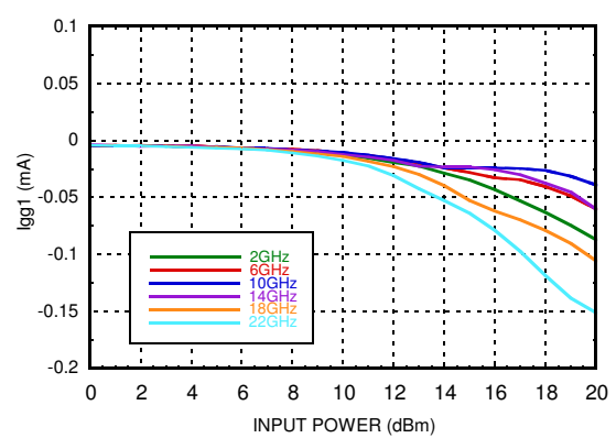
Igg1 vs. RF Input Power
