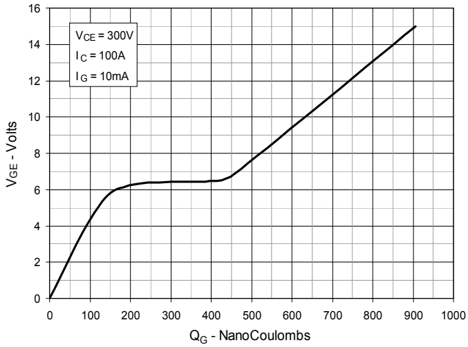
Fig. 7. Gate Charge
