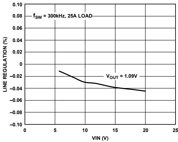
Figure 3. Line Regulation
