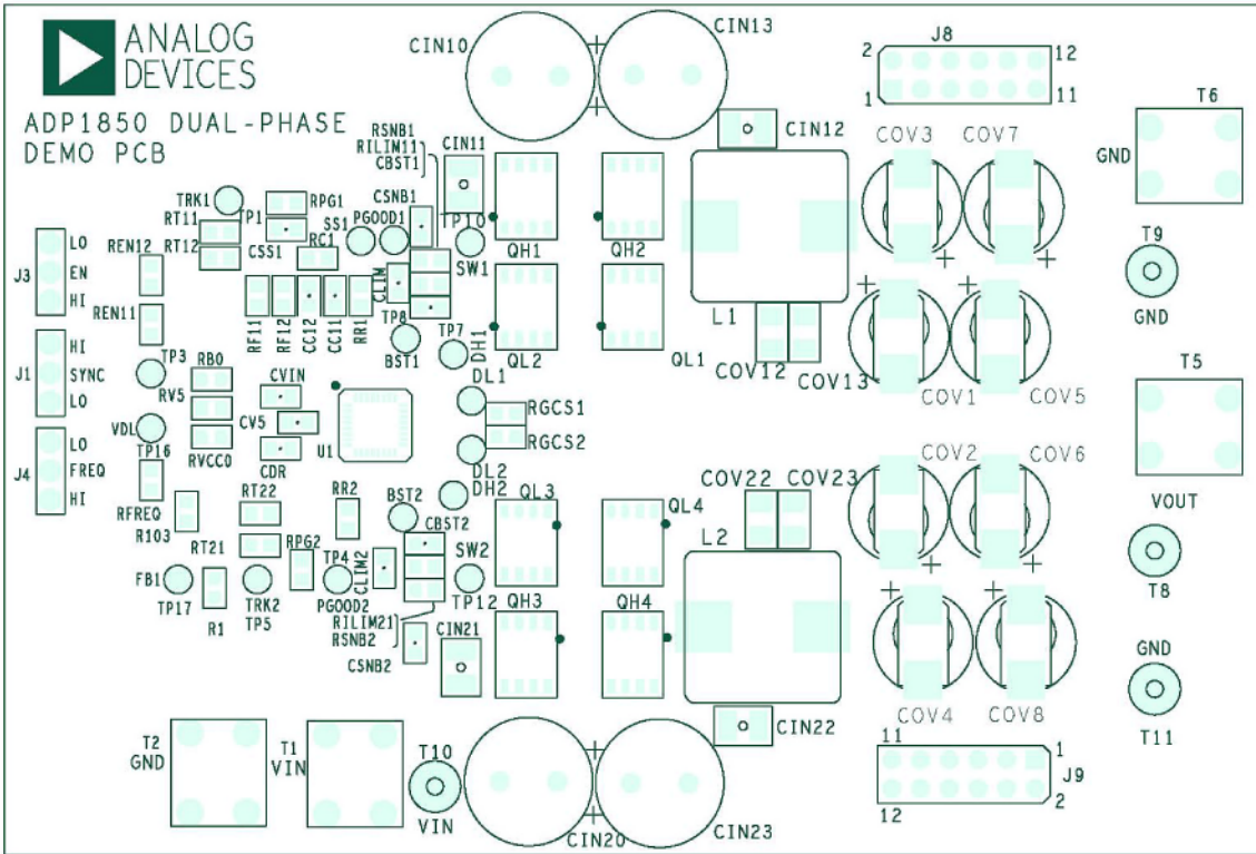
Figure 8. Top Silkscreen
