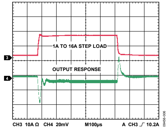
Figure 6. Step Load Transient, V OUT
