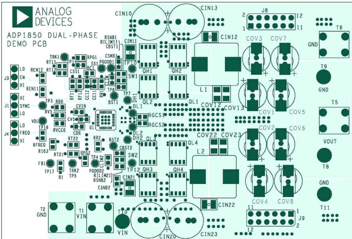
Figure 9. Top Layer
