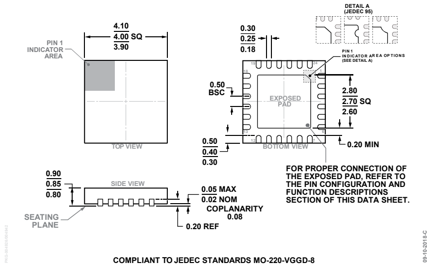
Figure 23. 24-Lead Lead Frame Chip Scale Package [LFCSP] 4 mm × 4 mm Body and 0.85 mm Package Height (CP-24-16) Dimensions shown in millimeters
