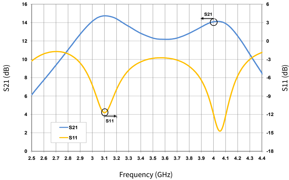
Figure 1. Small Signal S-Parameters vs Frequency measured in the CGH35015F-AMP V_{DD} = 28\text{ V} , I_{DQ} = 100\text{ mA}
