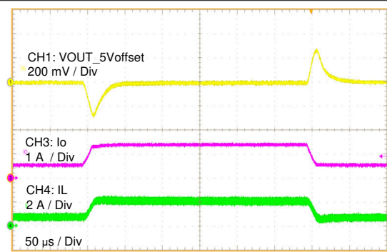
Figure 9-5. Load Sweep
