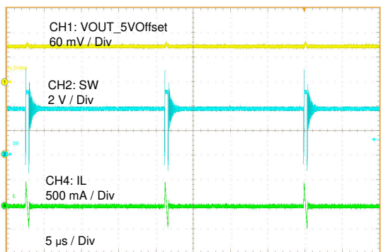
Figure 9-2. Steady 10 mA
