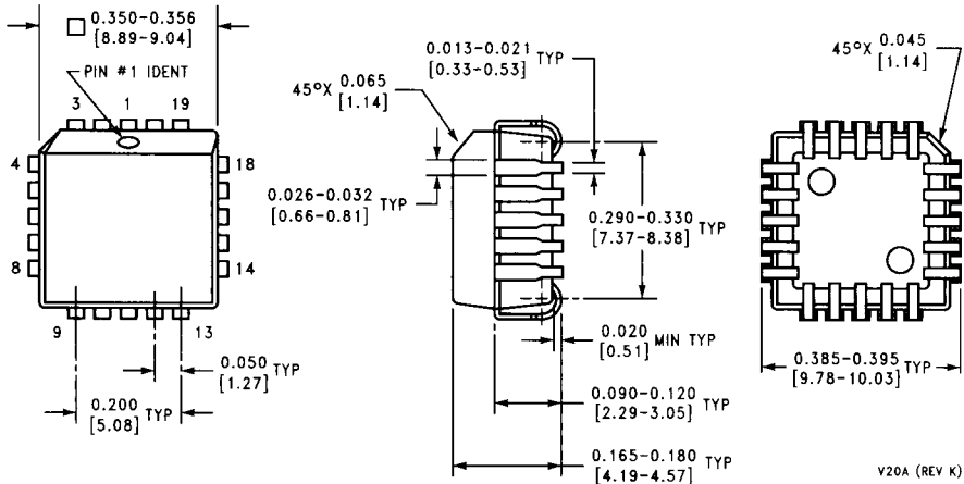
20-Lead Molded Plastic Leaded Chip Carrier NS Package Number V20A
