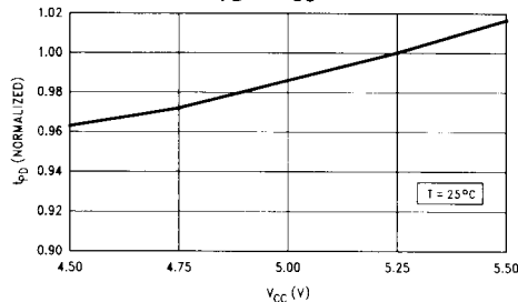
t_{PD} vs V_{CC}
