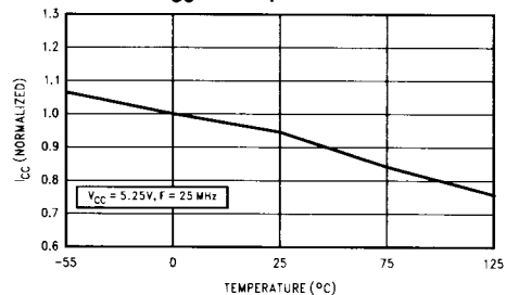
I_{CC} vs Temperature
