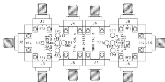
Figure 20. Evaluation Board Component Placement
