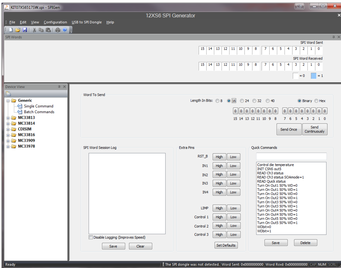
Figure 4. SPIGen GUI
