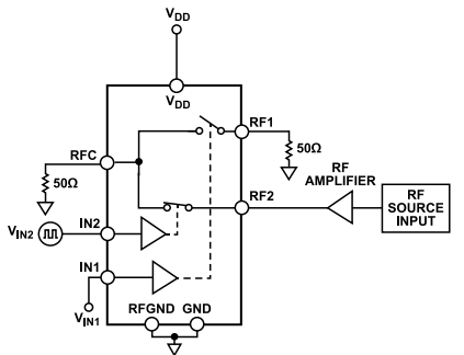
Figure 65. RF Hot Switching Setup
