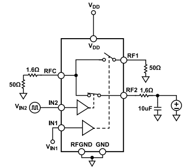
Figure 67. DC Hot Switching Setup
