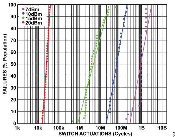
Figure 66. RF Hot Switching Probability Distribution on Log Normal (RF Power = Continuous Wave, Terminated into 50 Ω, TA = 25°C, VDD = 3.3 V)
