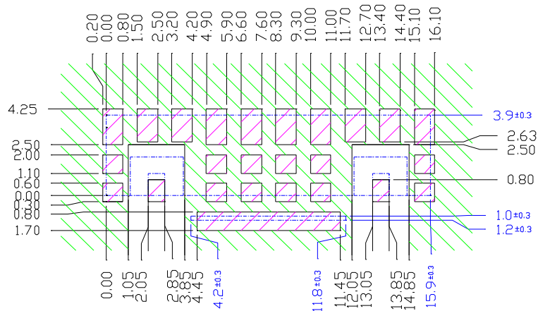
PCB Layout
