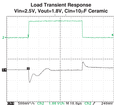
Cout = 10μF Tantalum (ESR~700mΩ) Ch1 – Vout (AC, 0.5V/div) Ch2 – Load Current (1A/div.)
