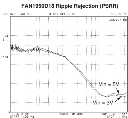
Vin = 3V and 5V Vout = 1.8V Iload = 1A Cin = Cout = 10μF/ 6.3V Tantalum PSRR – 10dB/div
