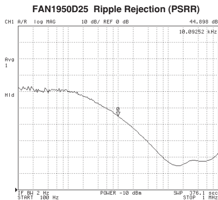
Vin = 5V Vout = 2.5V Iload = 1A Cin = Cout = 10μF/ 6.3V Tantalum PSRR – 10dB/div
