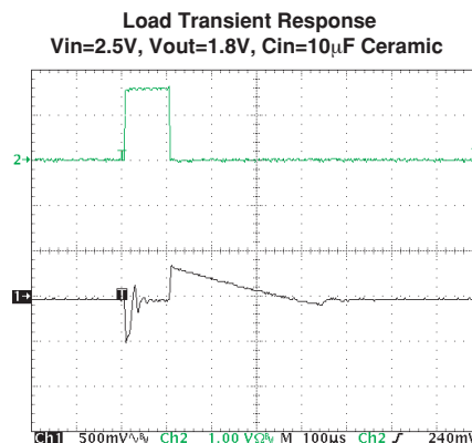
Cout = 10μF Ceramic Ch1 – Vout (AC, 0.5V/div.) Ch2 – Load Current (1A/div.)
