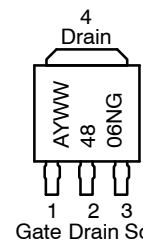
1 Gate 2 Drain 3 Source 4 Drain
