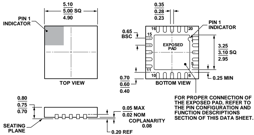
Figure 56. 20-Lead Lead Frame Chip Scale Package [LFCS P _WQ] 5 mm × 5 mm Body, Very Very Thin Quad (CP-20-9) Dimensions shown in millimeters
