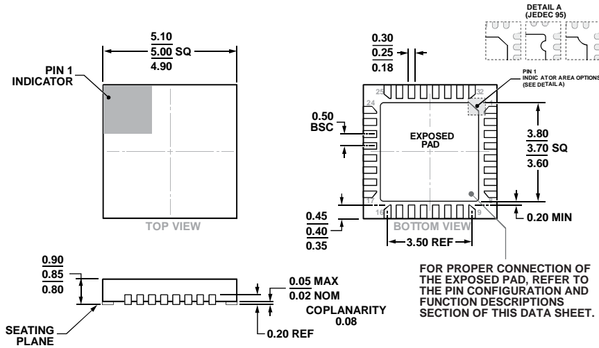
Figure 85. 32-Lead Lead Frame Chip Scale Package [LFCSP] 5 mm × 5 mm Body and 0.85mm Package Height (HCP-32-1) Dimensions shown in millimeters
