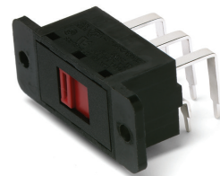
V80213SL08Q Horizontal Actuation DPDT
