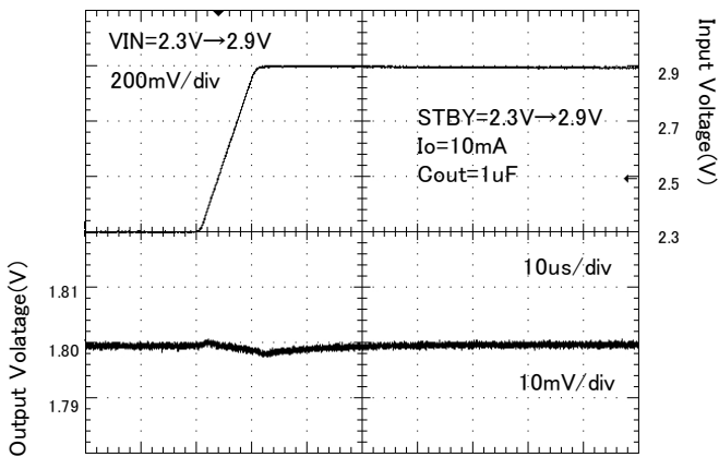
Figure 24. Line response ( Vin= 2.3V → 2.9V)
