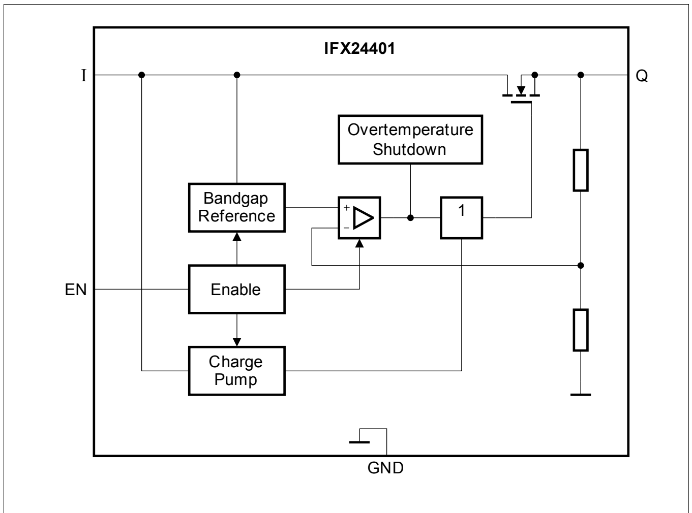
Figure 1 Block Diagram
