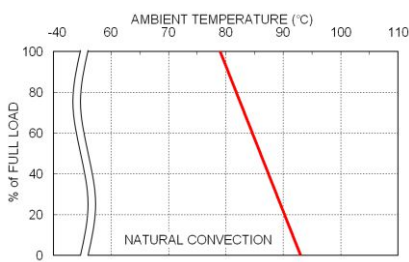
DFED20-48S05 Derating Curve
