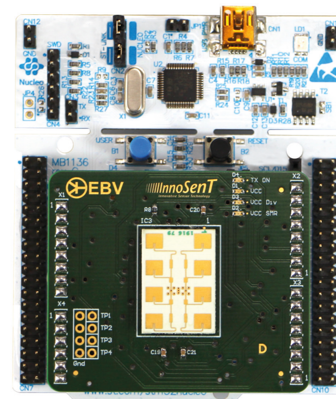
Figure 3: SMR-board and STM32 board connection
