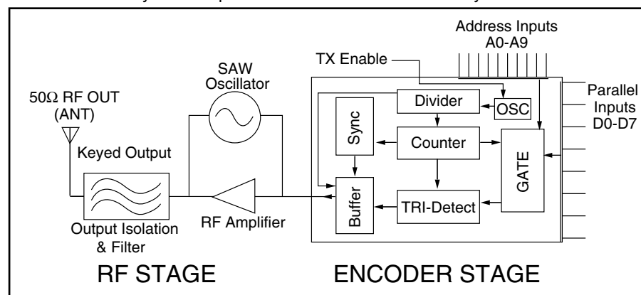
Figure 7: KH2 Series Transmitter Block Diagram
