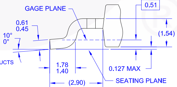
DETAIL A (ROTATED -90°) SCALE: 12X
