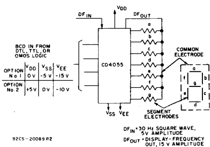
Fig. 20 — Single-digit liquid-crystal display.
