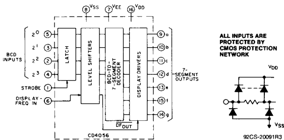
Fig. 3 - CD4056B functional diagram.
