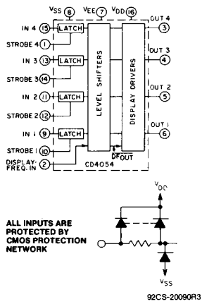
Fig. 1 - CD4054B functional diagram.
