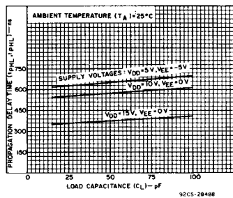
Fig. 5 - Typical propagation delay time vs. load capacitance for CD4055B and CD4056B.
