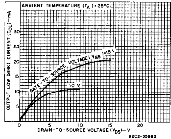
Fig. 8 - Typical n-channel output low (sink) current characteristics.
