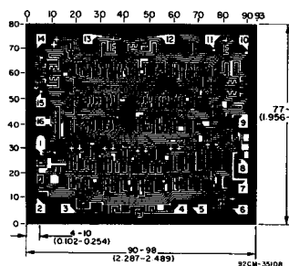
Dimensions and pad layout for CD4055BH
