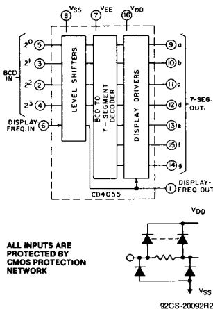
Fig. 2 - CD4055B functional diagram.
