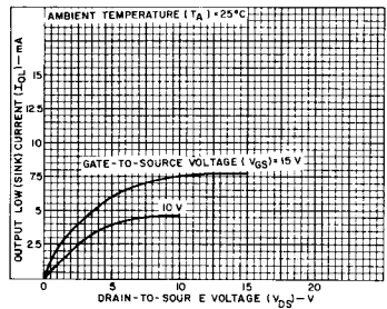
Fig. 9 - Minimum n-channel output low (sink) current characteristics.
