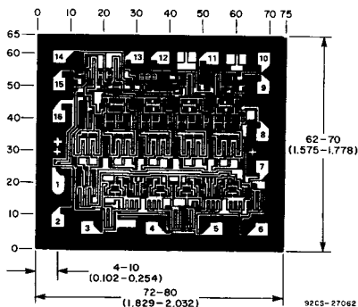
Dimensions and pad layout for CD4054BH.
