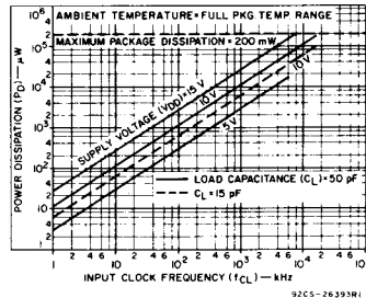
Fig. 7 - Typical input clock frequency vs. power dissipation.
