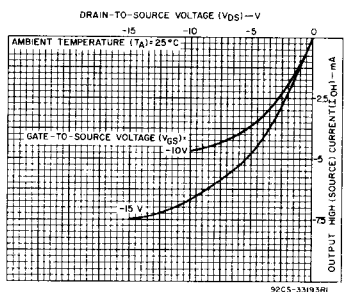
Fig. 13 - Minimum p-channel output high (source) current characteristics.
