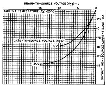
Fig. 10 - Typical p-channel output high (source) current characteristics.
