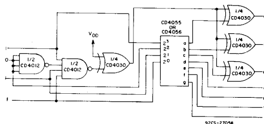
Fig. 21 — Conversion of "H" display to "F" display.
