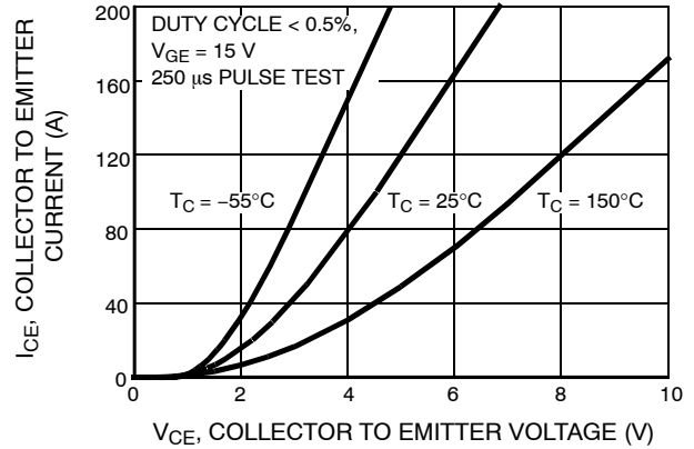
Figure 6. COLLECTOR TO EMITTER ON-STATE VOLTAGE
