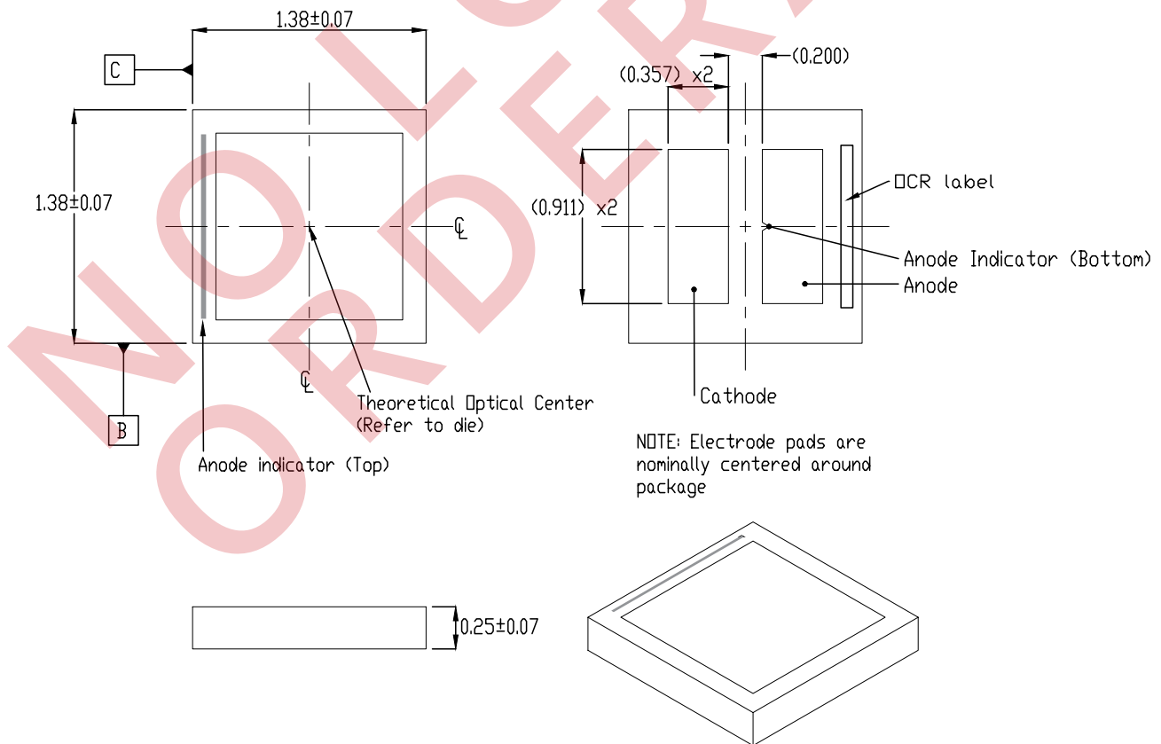
Figure 10. Mechanical dimensions for LUXEON CSP HL1.
