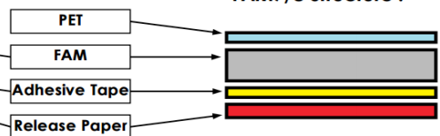
FAM7/8 Structure :
