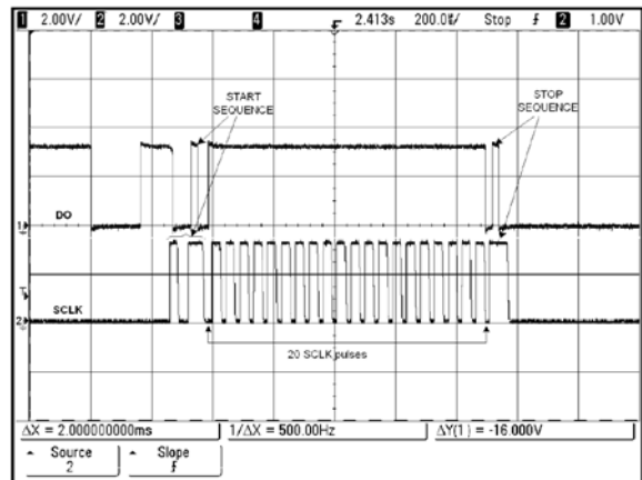
Figure 10. All Bits D19 through D0 = 1
