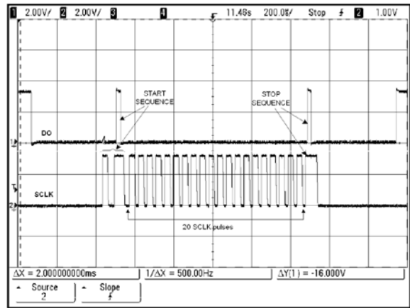
Figure 9. All Bits D19 through D0 = 0
