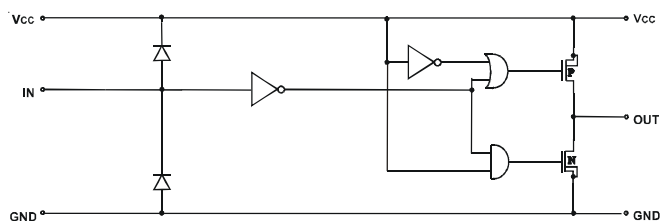
Figure 1C - IXDI409 (Inverting) Diagram
