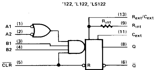
logic diagram
