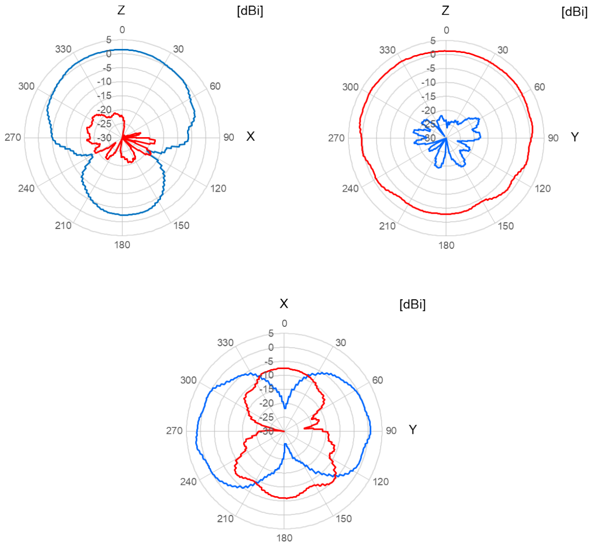
Radiation Pattern @2.45 GHz
