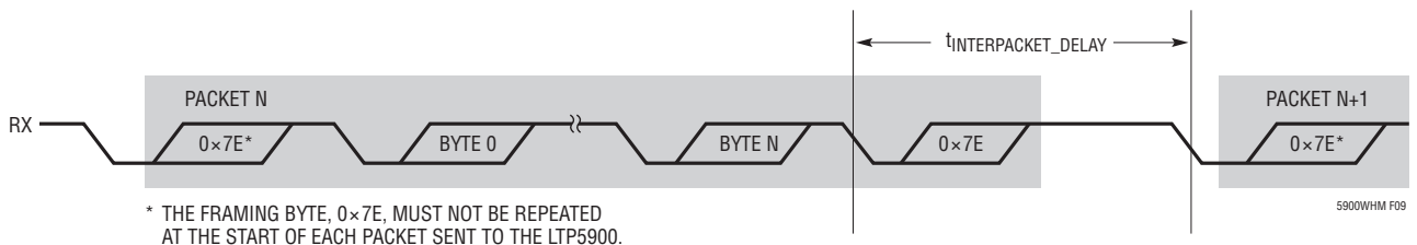
Figure 9. Packet Timing
