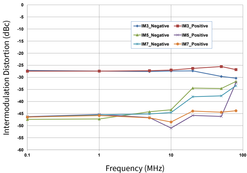
Figure 2. Intermodulation Distortion Performance vs. Tone Spacing V_{DD} = 40\text{ V}, \text{Frequency} = 8.2\text{ GHz}, \text{Output Power} = 44\text{ dBm} / 20\text{ W}
