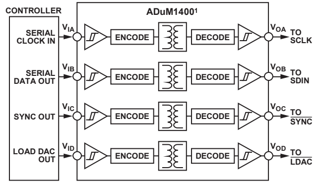
Figure 54. Isolated Interface
