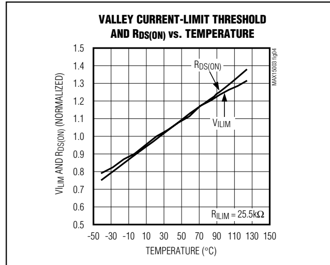
Figure 4. Current-Limit Trip Point and V RDS(ON) vs. Temperature
