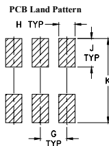
Suggested Layout, Tolerance to be within ±.002
