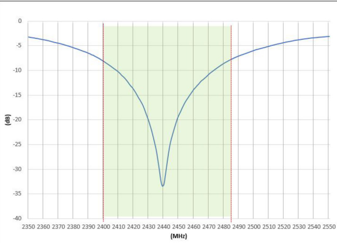
Return Loss
