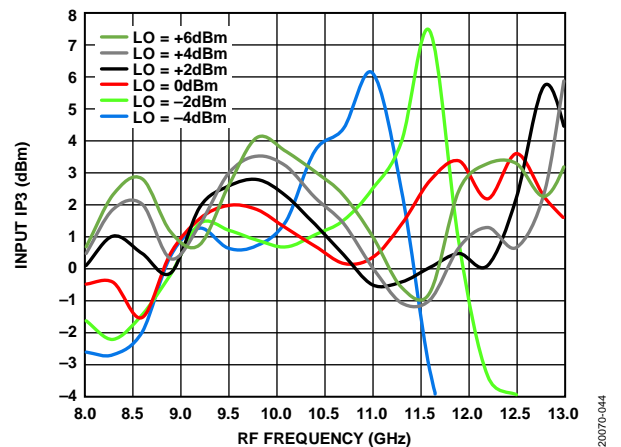
Figure 45. Input IP3 vs. RF Frequency at Various LO Powers, T A = 25°C
