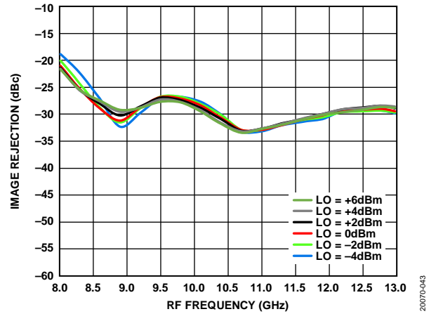
Figure 44. Image Rejection vs. RF Frequency at Various LO Powers, T A = 25°C
